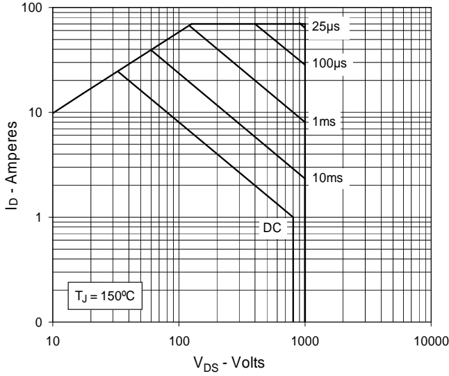
Fig. 12. Forward-Bias Safe Operating Area @ T_C = 25^\circ\text{C}
